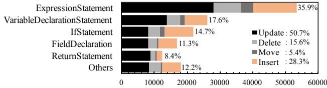
Fig. 7: Distributions of statement-level repair actions of patches.
